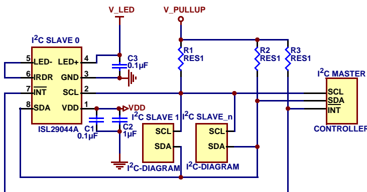
FIGURE 1. TYPICAL APPLICATION
